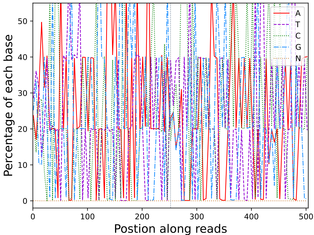
Base percentage along reads (R20210)
